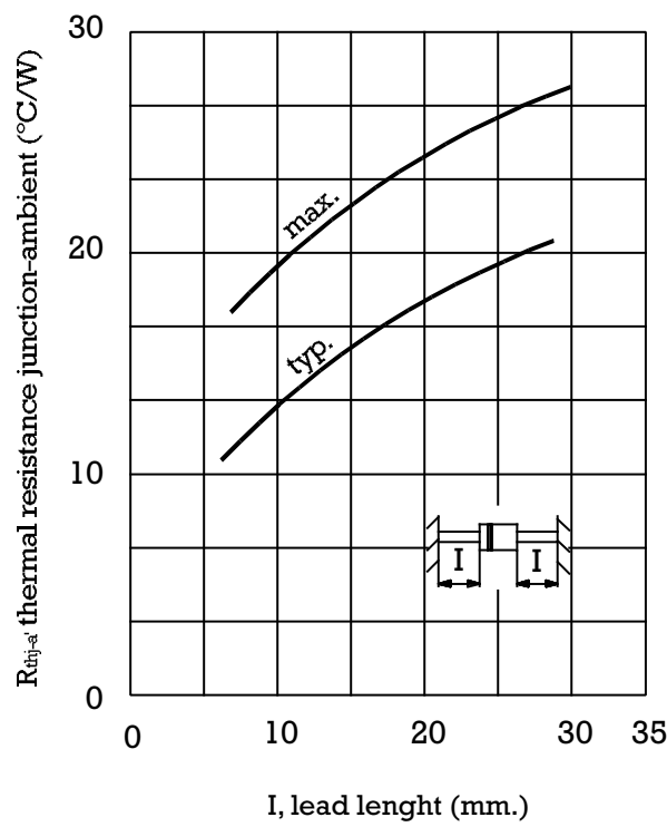
THERMAL RESISTANCE
