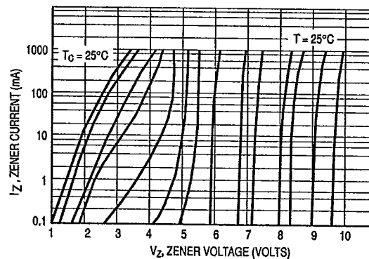
Figure 8. Zener Voltage versus Zener Current V<sub>Z</sub> = 3.3 thru 10 Volts
