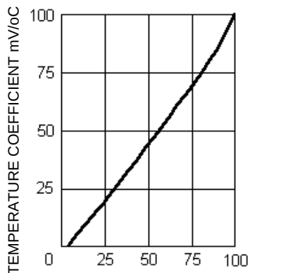
FIGURE 2 Temp. Coeff. vs. Zener Voltage
