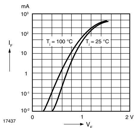
Figure 1. Forward characteristics
