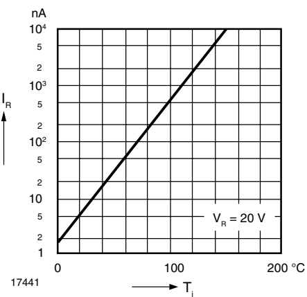
Figure 5. Leakage Current vs. Junction Temperature
