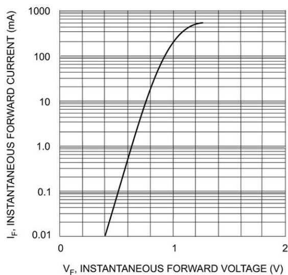
Fig. 2 Forward Characteristics
