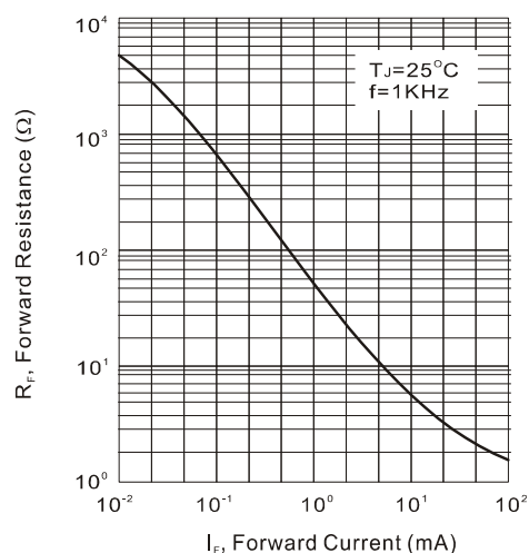
Fig.4 Dynamic Forward Resistance Versus Forward Current
