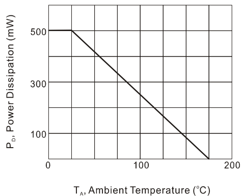
Fig.1 Derating Curve
