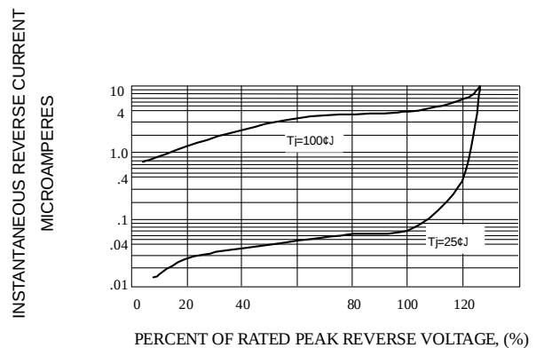
Fig. 5-TYPICAL REVERSE CHARACTERISTICS
