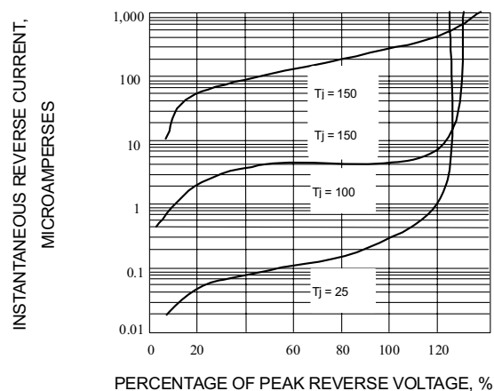
Fig. 2-TYPICAL REVERSE CHARACTERISTICS
