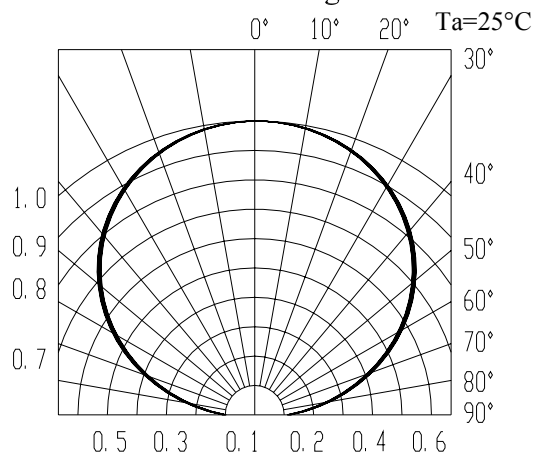
Radiation Diagram
