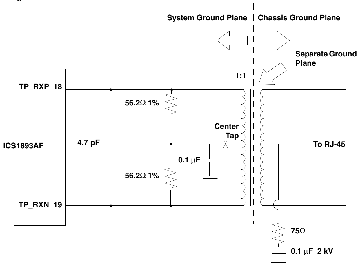
Figure 6-2. ICS1893AF Receiver Twisted Pair
