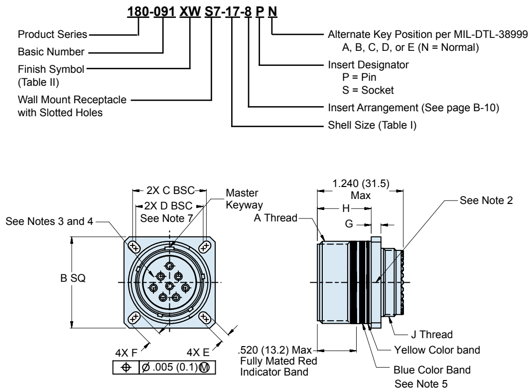
S7 - WALL MOUNT RECEPTACLE WITH SQUARE FLANGE AND SLOTTED HOLES
