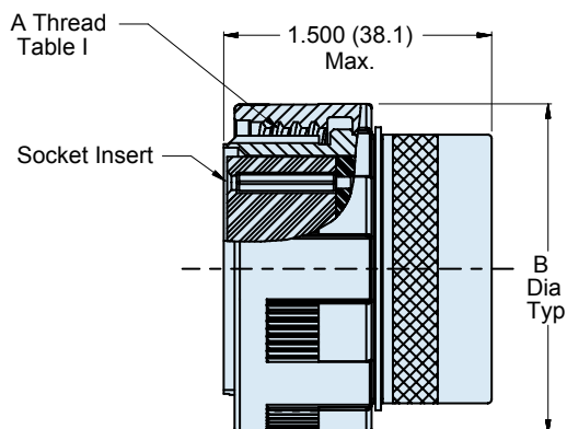
06 PLUG ASSEMBLY U.S. PATENT NO. 5,960,137
