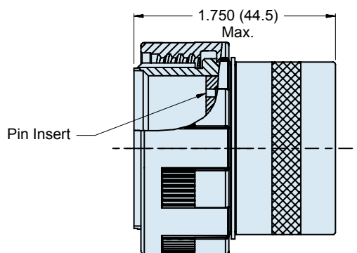
06 PLUG ASSEMBLY U.S. PATENT NO. 5,960,137
