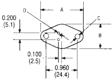
TO-66
