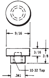
FLAT FACED Class 1 SE-3099-1 Part No. 170-3099-1 Class 2 SE-3099 Part No. 170-3099 Class 3 SE-3111 Part No. 170-3111 ZIRC SE-3099-Z Part No. 170-3099-Z
