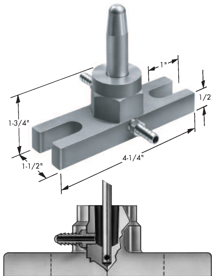
Size 2 PM Holder (3/4-in. mounting bolts)
