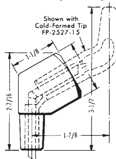
AD-55-30, for 5 RW Tip, Part No. 190-9553
