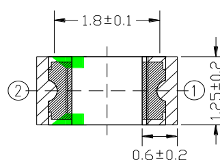
Recommend Soldering Pad
