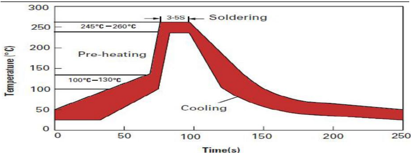
recommended curve
