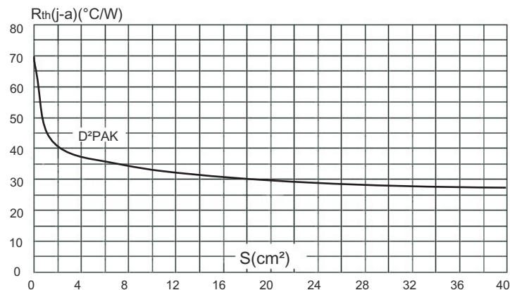
Fig.11 D 2 PAK thermal resistance junction to ambient versus copper surface under tab (printed circuit FR4, copper thickness: 35 \mu m )
