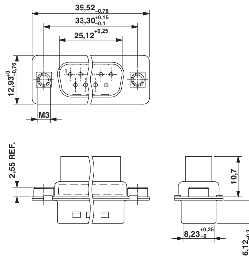
Dimensioned drawing
