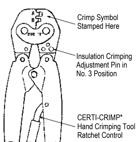
Pin
