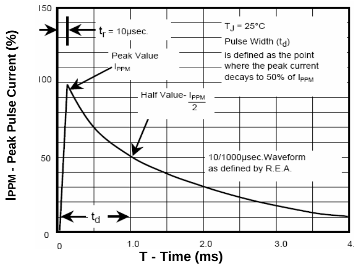
Fig.3- Pulse Waveform
