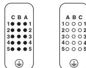
Connector pin assignment, connection side: left pin, right socket
