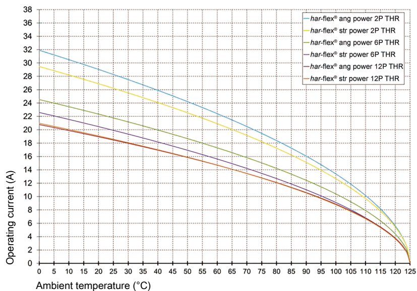
Derating curve 80%
