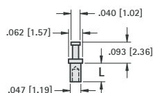
Staking Tool 1528-TL
