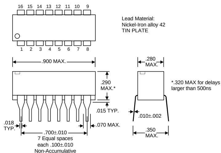
Package Dimensions
