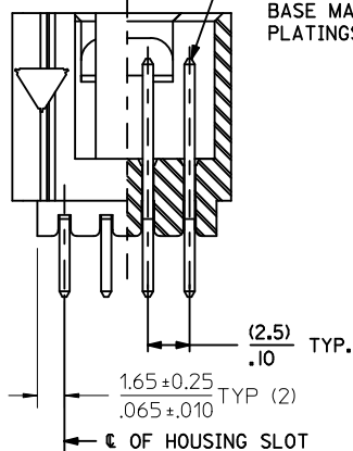
SECTION E-E
