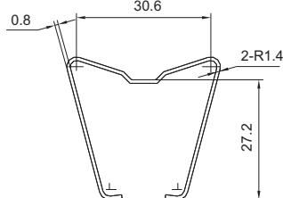
14FF-H2(metallic retainer)
