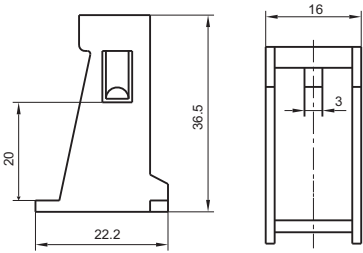
140F-H1(Plastic retainer)
