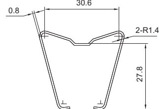
14FF-H3(metallic retainer)
