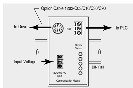
GD1/GD2 – Typical Configuration
