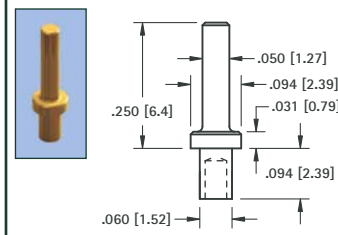
.050 (1.3) PIN - SWAGE MOUNT
