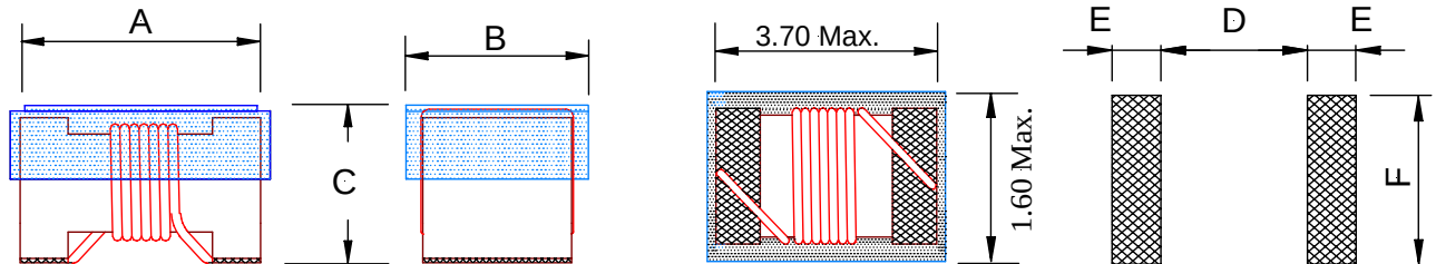
Land Pattern
