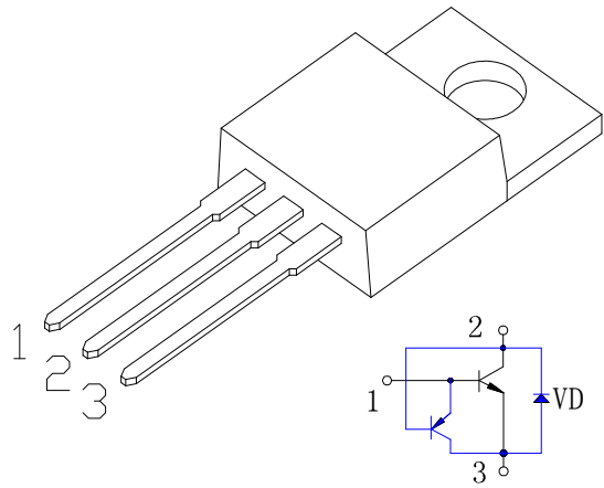
1 Base(B) 2 Collector(C) 3 Emitter(E)
