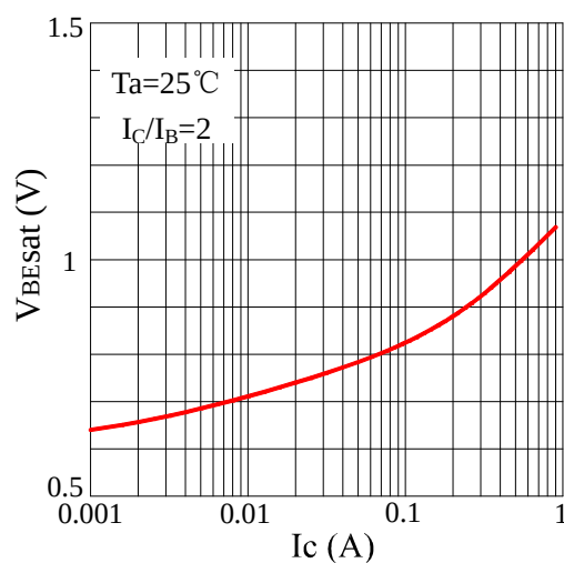
Fig4 V_{BEsat} - I_C
