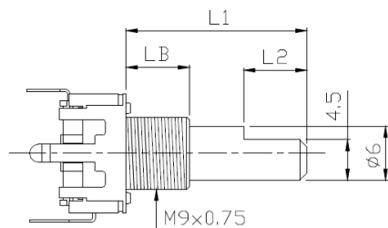
Flatted Shaft
