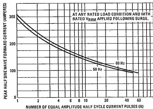
Fig. 21 - Maximum Non-Repetitive Surge Current Vs. Number of Current Pulses, 16F Series
