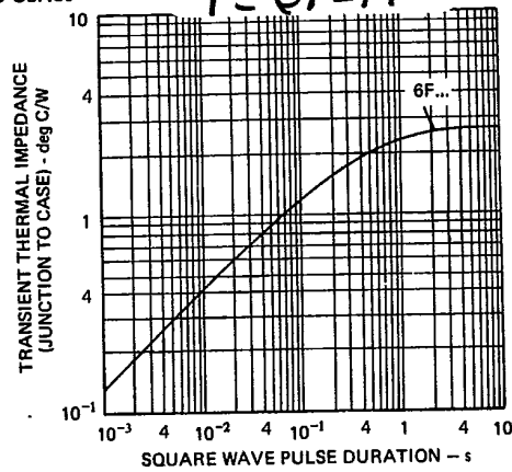
Fig. 6 - Maximum Transient Thermal Impedance, Junction-to-Case Vs. Pulse Duration, 6F Series
