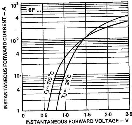
Fig. 5 - Maximum Forward Voltage Vs. Forward Current, 6F Series
