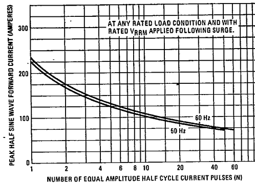
Fig. 14 - Maximum Non-Repetitive Surge Current Vs. Number of Current Pulses, 12F Series
