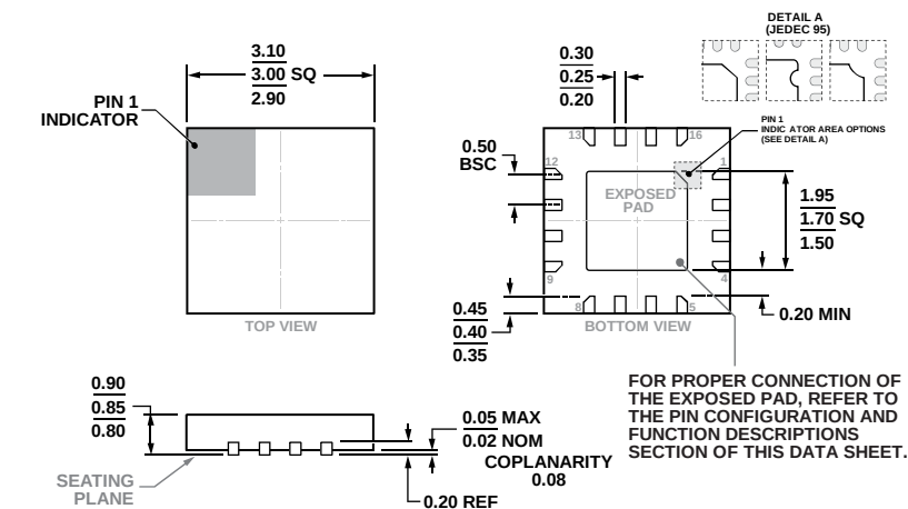
Figure 25. 16-Lead Lead Frame Chip Scale Package [LFCSP] 3 mm x 3 mm Body and 0.85 mm Package Height (HCP-16-1)
