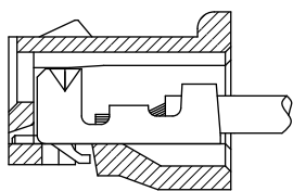
TERMINAL ASSEMBLY DRAWING
