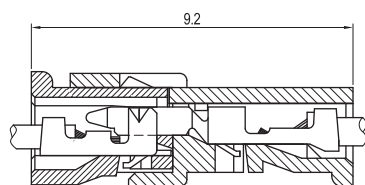
TERMINAL ASSEMBLY
