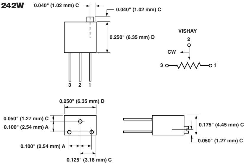
FIGURE 1 - SCHEMATIC AND DIMENSIONS in inches (millimeters)
