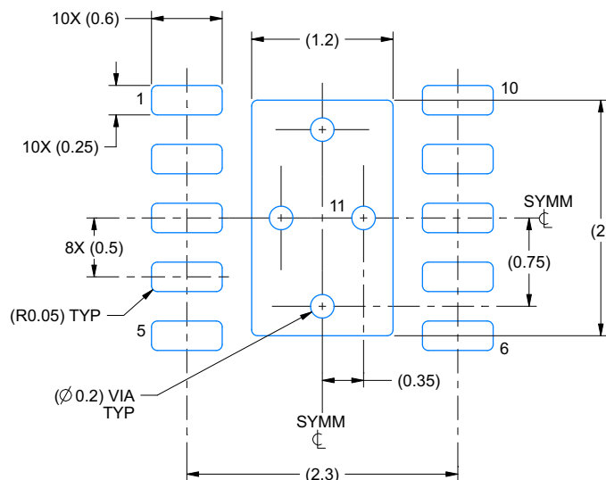
LAND PATTERN EXAMPLE SCALE:20X
