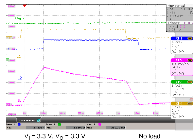
Figure 24. Switching Waveforms, PFM Buck Operation
