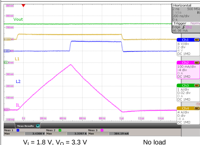
Figure 22. Switching Waveforms, PFM Boost Operation
