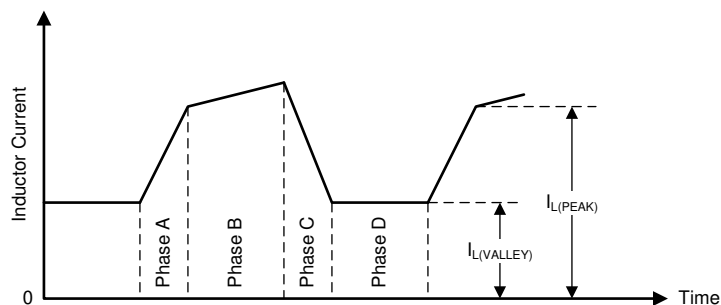
Figure 4. Inductor Current Waveform when V_I > V_O (CCM)
