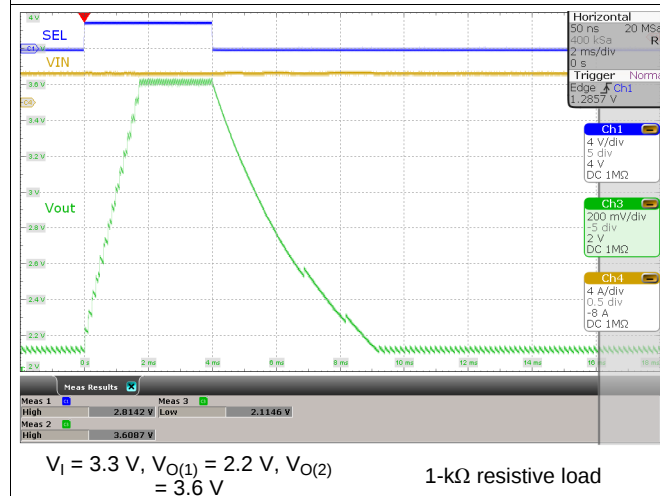
Figure 26. DVS Behavior at Light Load
