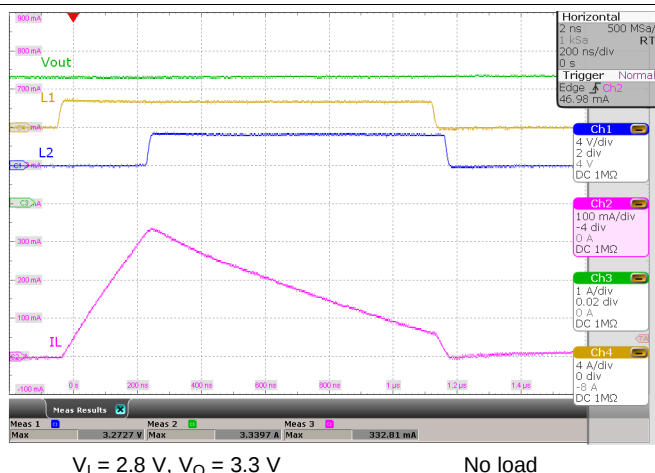
Figure 23. Switching Waveforms, PFM Buck-Boost Operation
