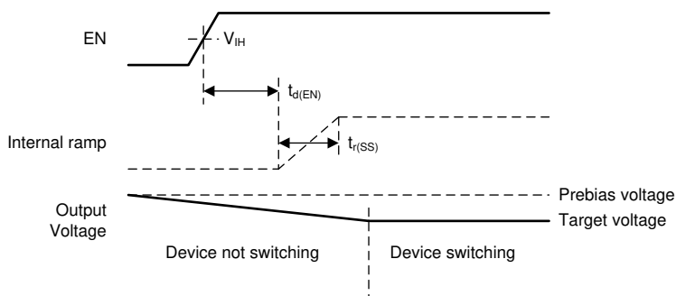
Figure 11. Start-Up Behavior into Prebiased (High) Output
