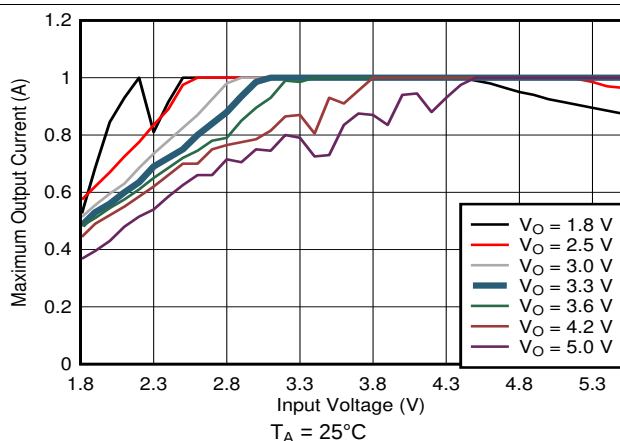
Figure 18. Typical Output Current Capability versus Input Voltage
