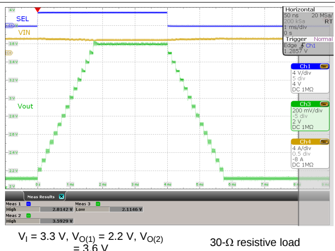
Figure 27. DVS Behavior at High Load
