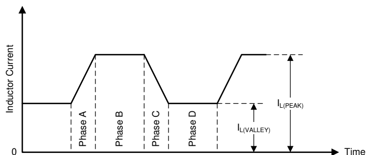
Figure 5. Inductor Current Waveform when V_I = V_O (CCM)
