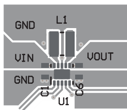
Figure 28. PCB Layout Example
