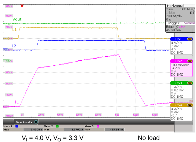
Figure 25. Switching Waveforms, PWM Boost Operation
