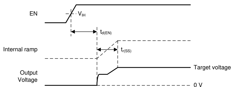
Figure 8. Start-Up Behavior
