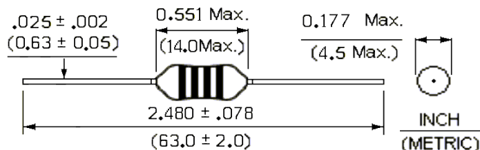
Mechanical drawing
