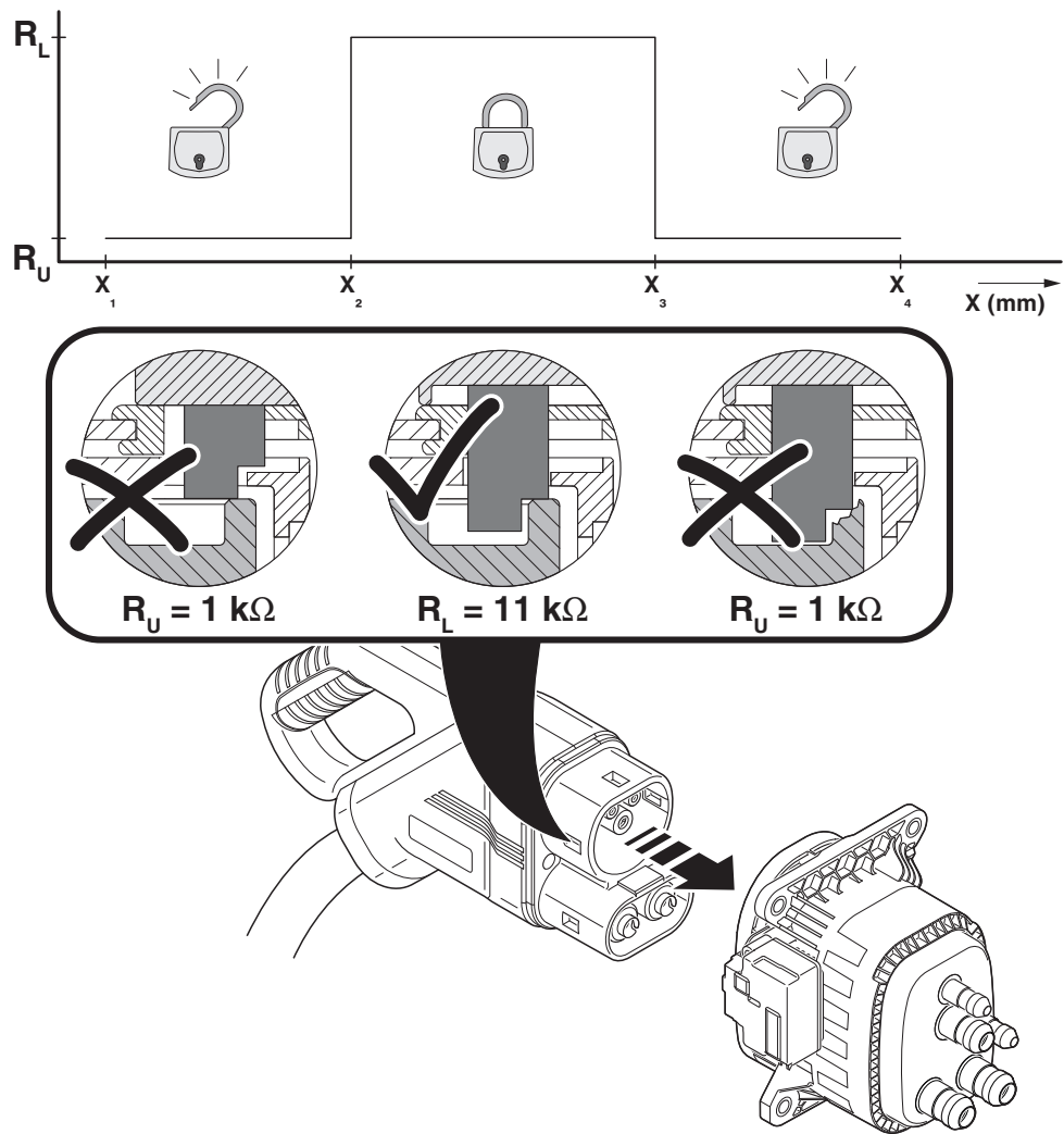
Connection diagram
