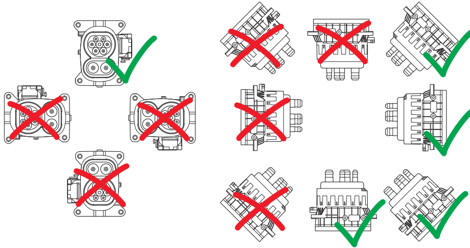
Connection diagram
