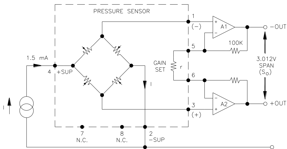
APPLICATION SCHEMATIC
