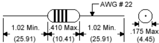
Mechanical drawing
