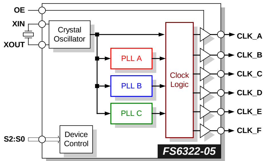
Figure 2: Block Diagram
