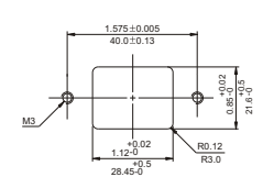
SUGGESTED MOUNTING CUTOUT
