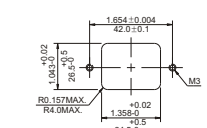
SUGGESTED MOUNTING CUTOUT (MOUNTING FROM REVERSE)
