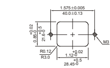
SUGGESTED MOUNTING CUTOUT (MOUNTING FROM FRONT)
