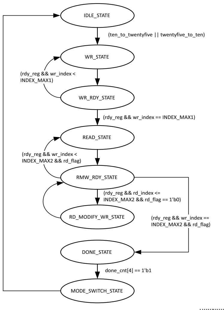
Figure 5-6: State Transition Diagram for Runtime Switchable DRP Operation without AN/LT
