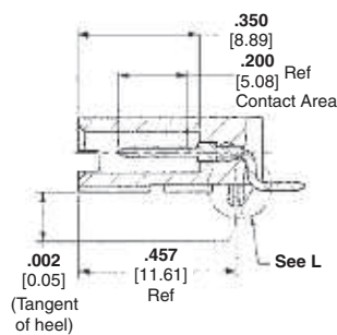
Section K-K
