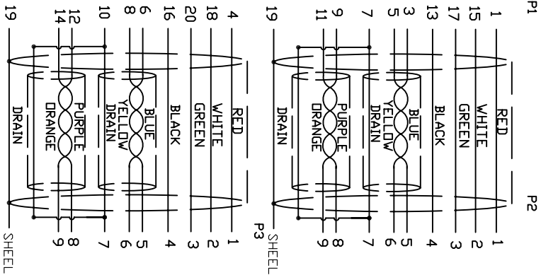
1.Wiring Diagram.
