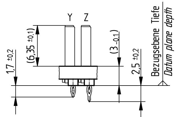
Kontaktversionen, Schirmmesser Contact Selection Options, Shielding Contacts
