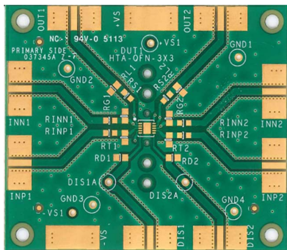
Figure 1. Evaluation Board, Component Side
