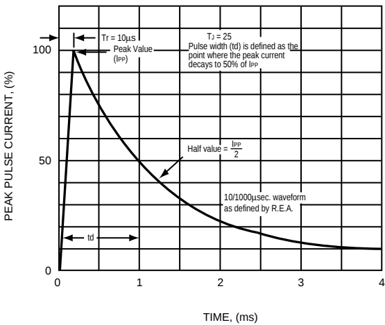
FIG. 4 - PULSE WAVEFORM
