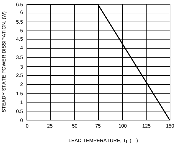
FIG. 2- STEADY STATE POWER DERATING CURVE
